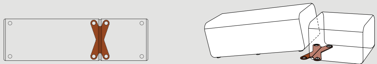
XOS-X-0003 SEAT + SEAT CONNECTOR
