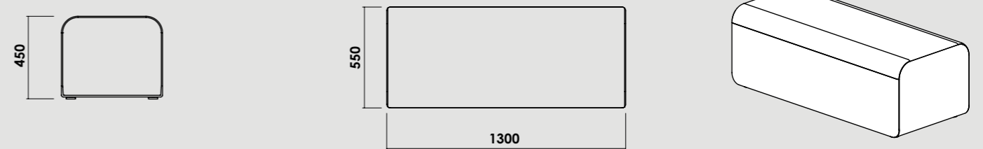
XOS-L-1300 XOXO LOOSE - INNER CURVE SEAT
