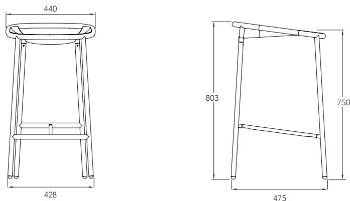
Bar Stool 750mm seat height
