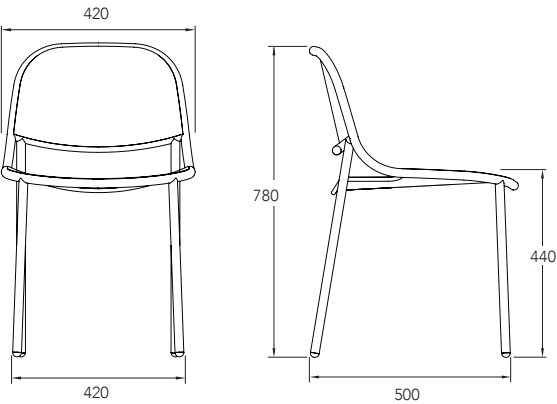
Chair 420w x 500d x 780h
