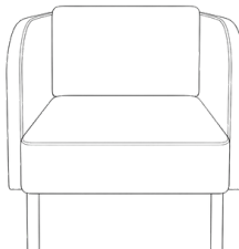
Single Seater 820 H / 850 W / 800 D / 440 SH
